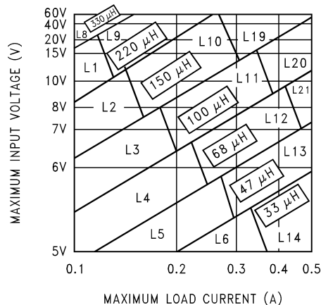
Figure 27. LM2594xx 3.3-V
