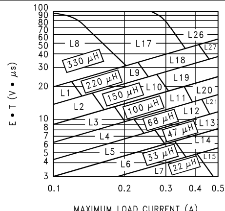
Figure 30. LM2594xx Adjustable Voltage
