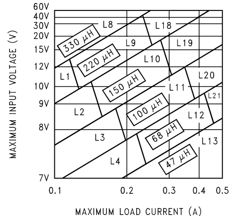
Figure 28. LM2594xx 5-V
