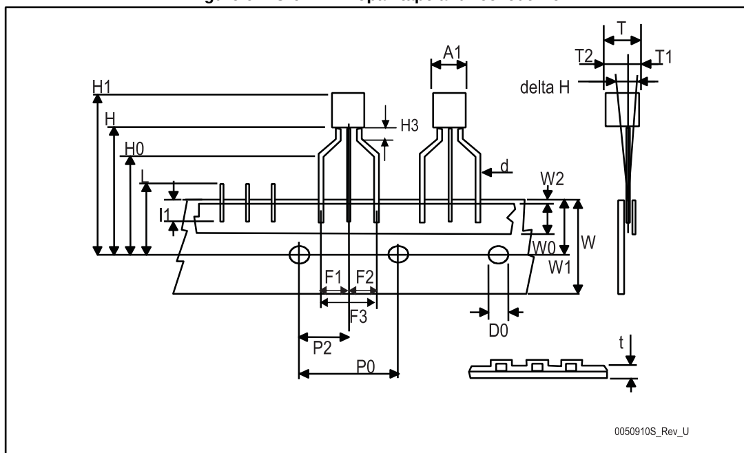
Figure 6: TO-92 Ammopak tape and reel outline
