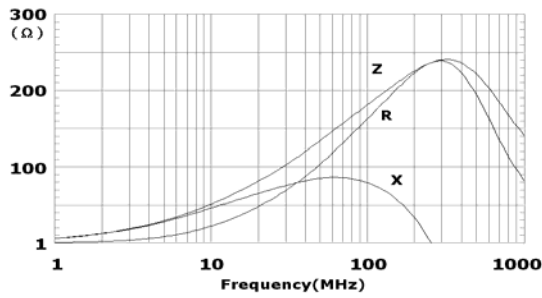
EBMS160808A221
