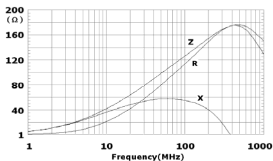
EBMS160808A121
