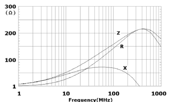
EBMS160808A151
