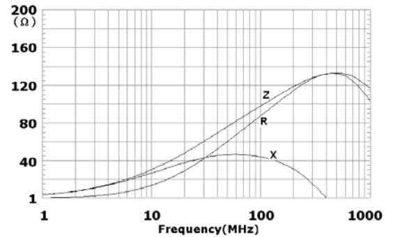
EBMS160808A101
