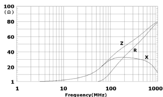
EBMS160808B300
