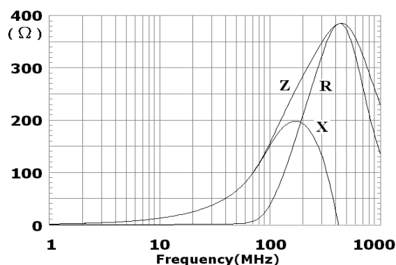
EBMS160808B151
