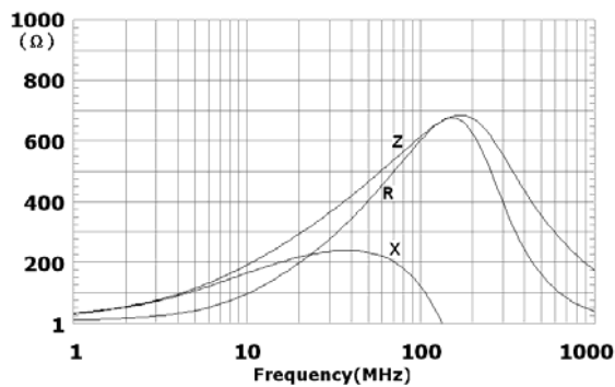
EBMS160808A601
