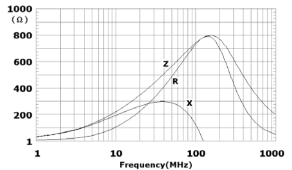
EBMS160808A751
