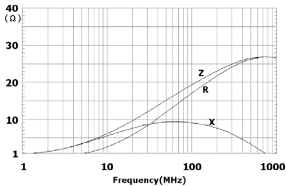
EBMS160808A520
