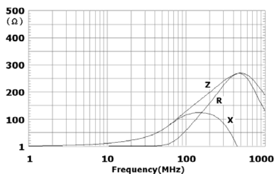
EBMS160808B121
