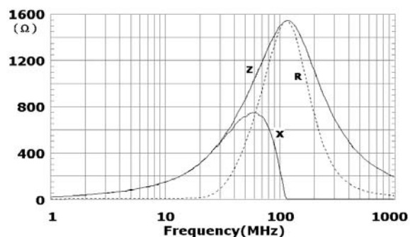
EBMS160808B300
