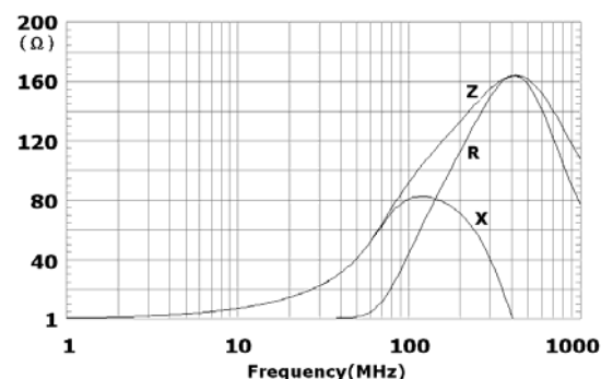
EBMS160808B151
