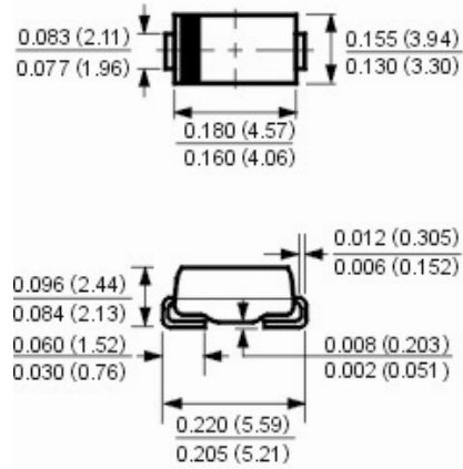
DO-214AA(SMB)
