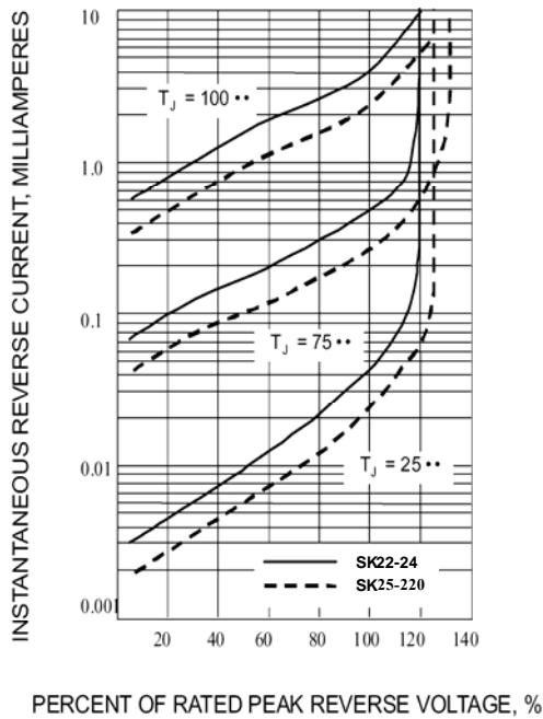
Fig. 3-TYPICAL REVERSE CHARACTERISTICS
