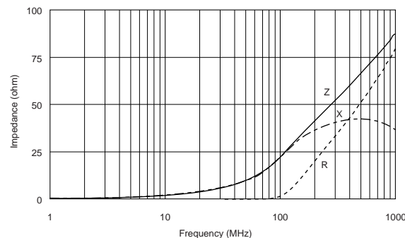
BLA2ABB220SN4
