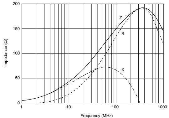
BLM21AG151SN1
