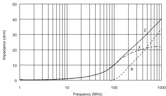
BLA2ABB100SN4
