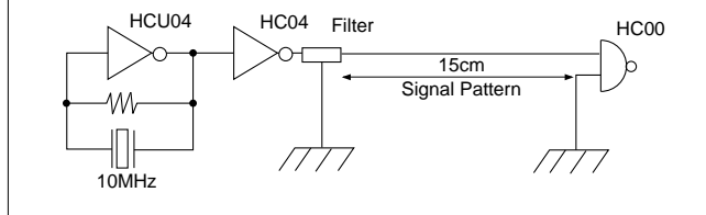
[Testing Circuit]
