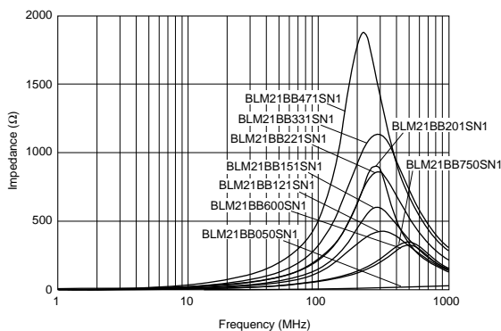
BLM21BB Series
