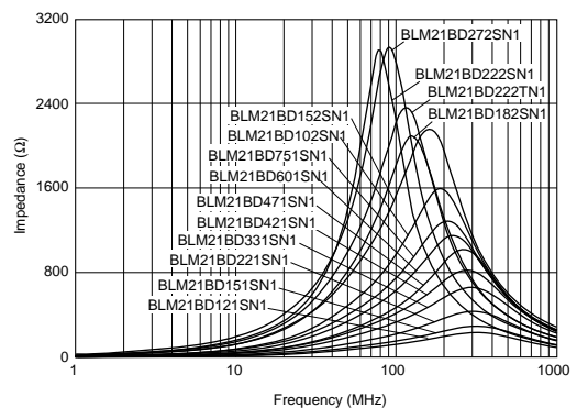
BLM21BD Series
